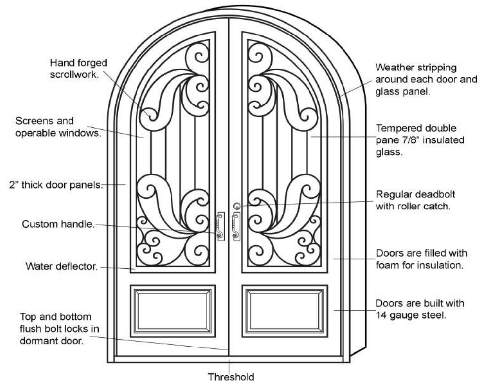
Cross section of standard door with special frame.
